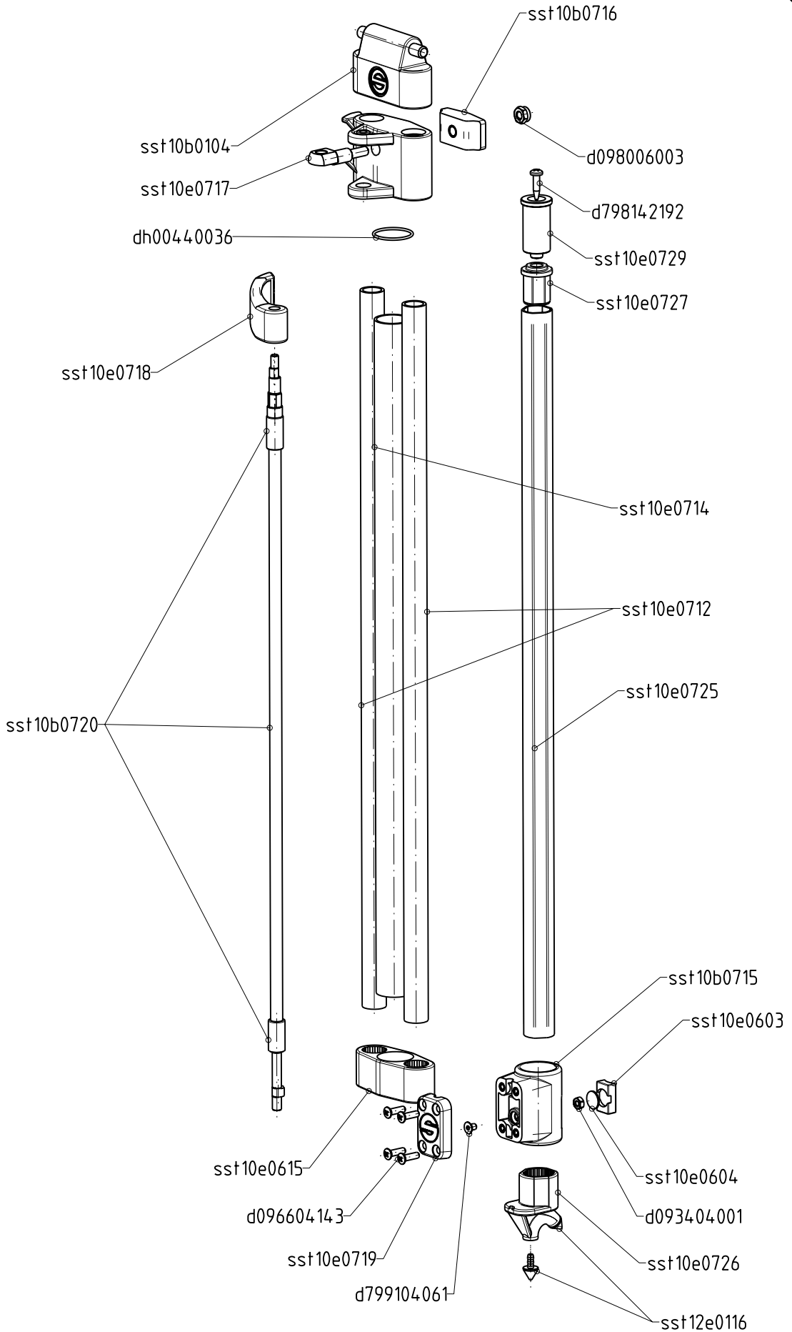
Dreibein / Tripod SpeedLock 75 sst10p0700
