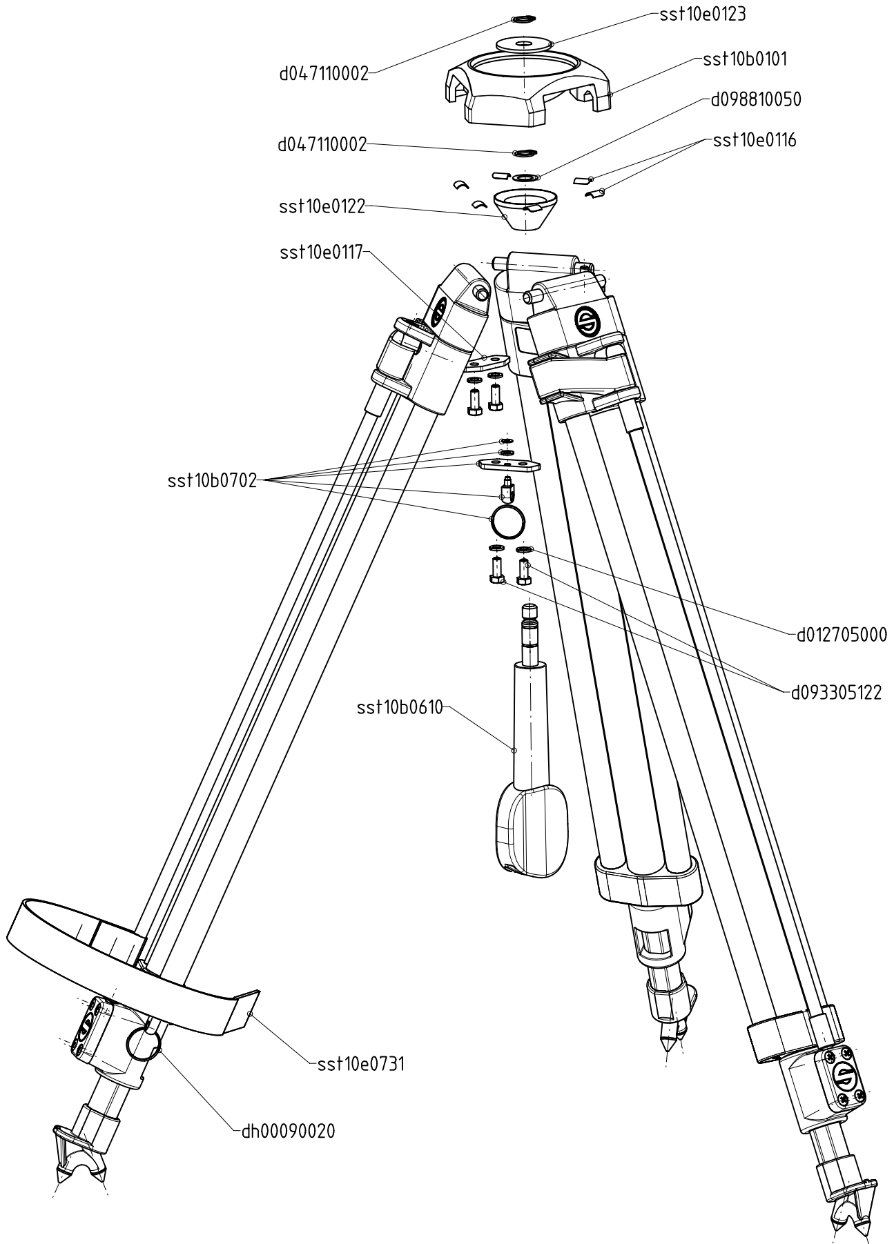
Dreibein / Tripod SpeedLock 75 sst10p0700
