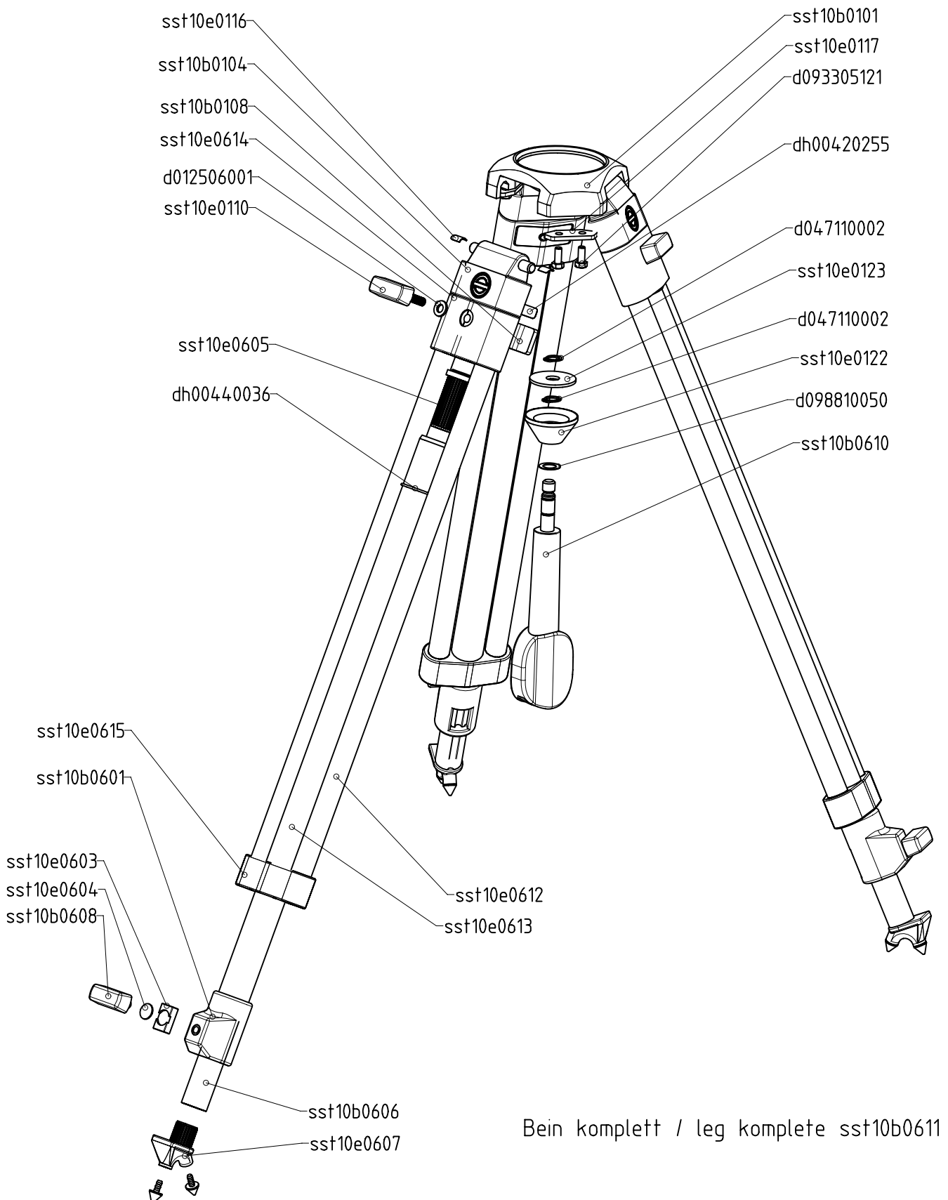
Dreibein / Tripod ENG 75 / 2 D sst10p0600
